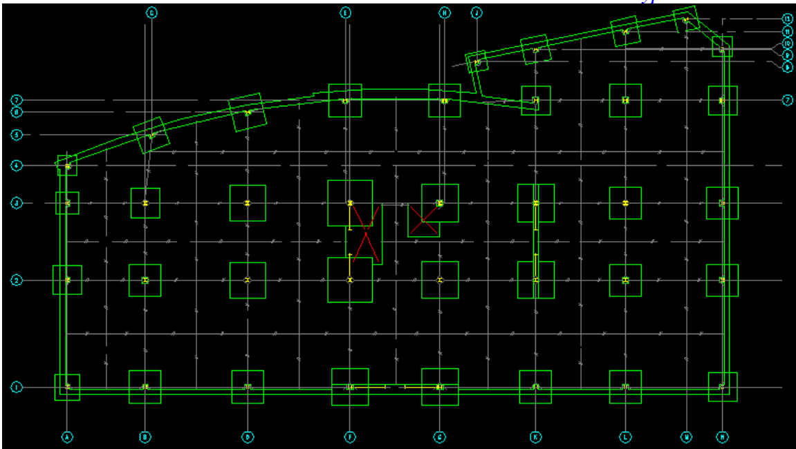
Foundation Plan
